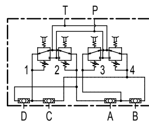
HYDRAULIC DIAGRAM HYDRAULIKSCHEMA
