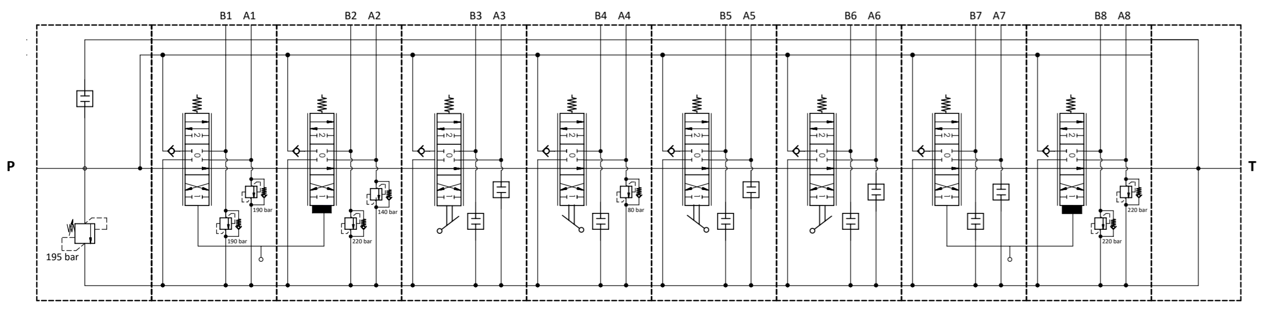
HYDRAULIC DIAGRAM
